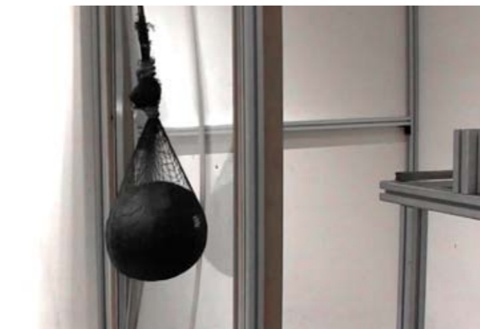
STRUCTURAL STABILITY TEST A ball up to the weight of 50kg is launched into the enclosure to ensure rigidity if there is a fall.
